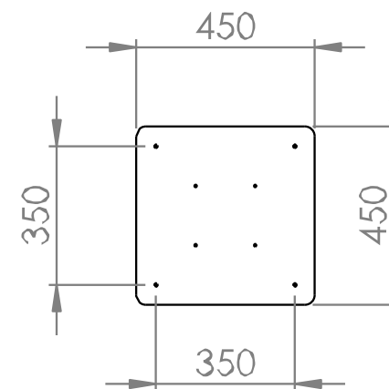
FLOOR PLATE
