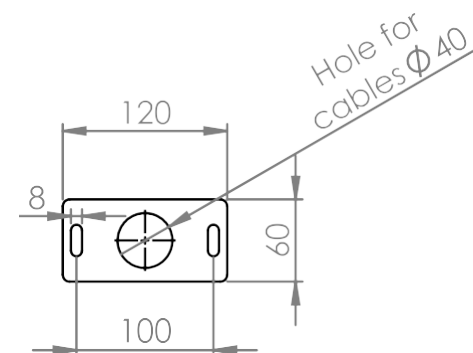
CEILING PLATE
